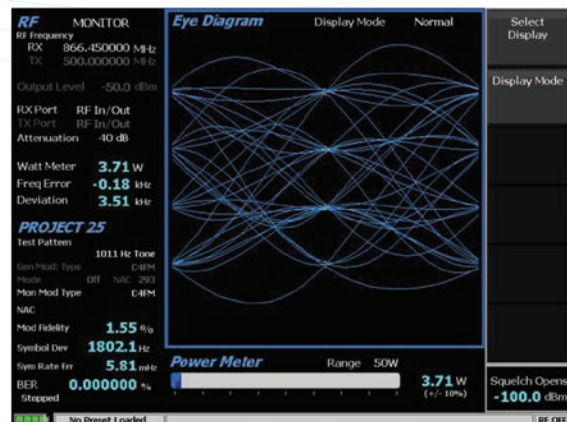
APCO P25 Phase1 Eye Diagram
